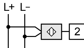
Muting sensor S2
