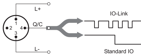
Fig. 22: 3-conductor physics of IO-Link
