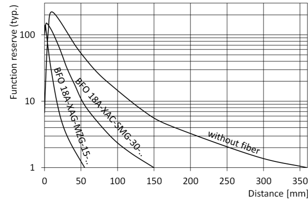
Fig. 6: Function reserve depending on distance BFB M18M-011-P-S4, Reference: white material, 90% remission, 100 x 100 mm 2
