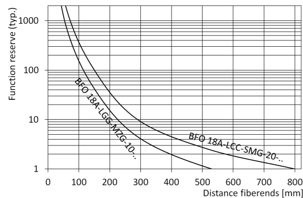
Fig. 8: Function reserve depending on distance between the fiber optics for BFB M18M-011-P-S4
