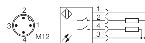
Fig. 5: Pin assignment M12, connection diagram
