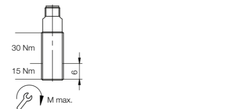
Fig. 3: Tightening torque
