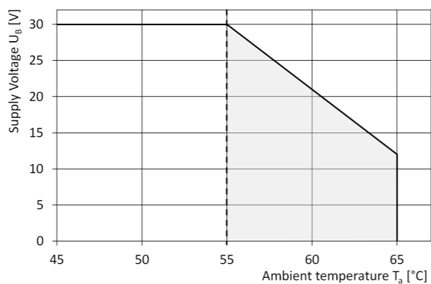
Fig. 11: Extended temperature range for use with lower supply voltage
