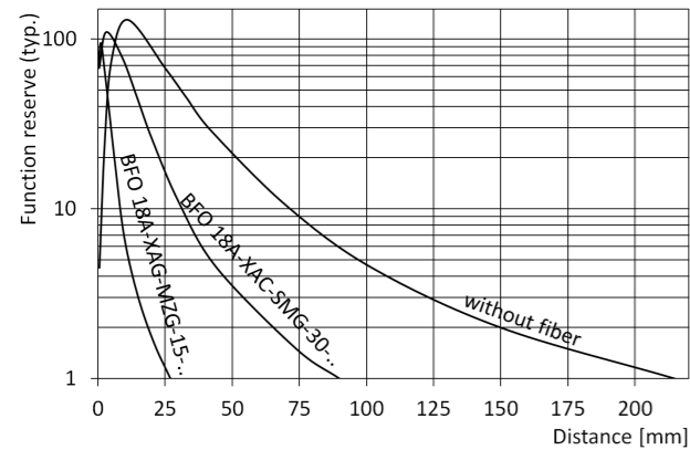
Fig. 7: Function reserve depending on distance BFB M18M-012-P-S4, Reference: white material, 90% remission, 100 x 100 mm 2
