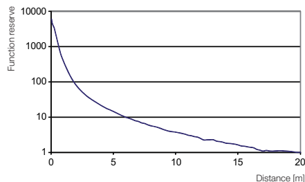
Fig. 7: Function reserve depending on distance, Reference material white, 90% remission, 200 x 200 mm 2
