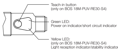
Fig. 3: Display and operating elements
