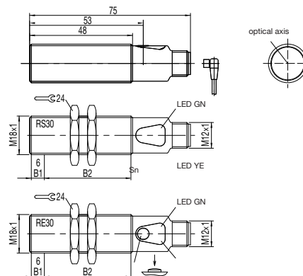
Fig. 4: Dimensions, tightening torque B1 = 15 Nm, B2 = 30 Nm
