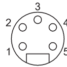
Fig. 5-1: Top view of 7/8" socket (left) and plug (right)
