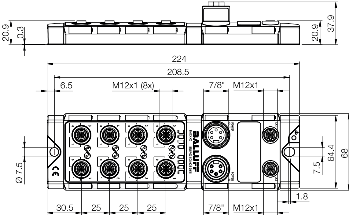
Fig. 4-1: Dimensions, design and function
