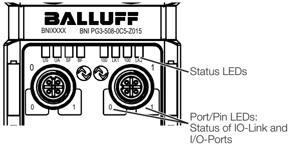
Fig. 4-3: Display elements
