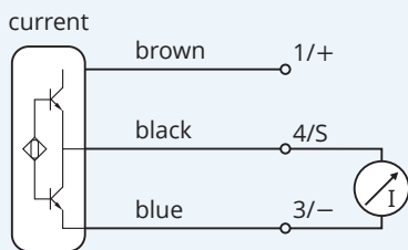
Wiring diagram
