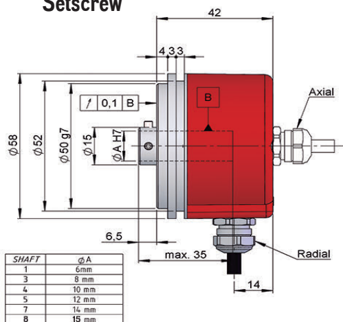
Drawing mechanical option type 2, blind hollow shaft type 5, connection type 3
