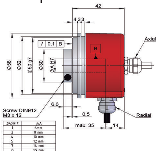
Drawing mechanical option type 1, blind hollow shaft type 5, connection type 3
