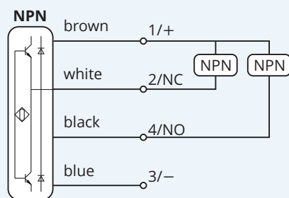
Wiring diagram
