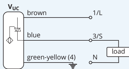
Wiring diagram
