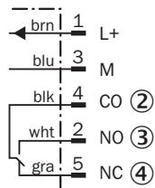
Receiver
