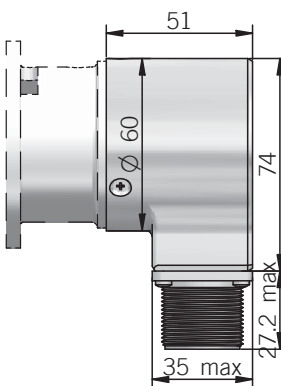
Dimensions with metal cover radial output
