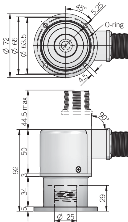
Dimensions with metal cover radial output
