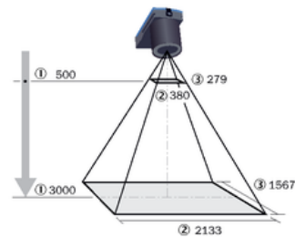
Figure 31: Field of view V2D8512R-xxxxxxx, focal length: 16 mm
