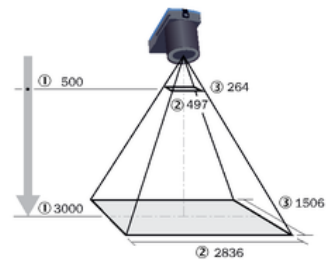
Figure 27: Field of view V2D8509R-xxxxxxxxx, focal length: 12 mm
