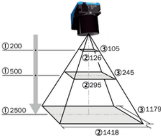
Fig. 4: Field of view of V2D8305R-xxxxxxxxx, focal length: 12 mm
