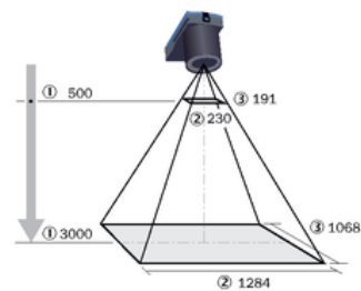
Figure 25: Field of view V2D8505R-xxxxxxxx, focal length: 16 mm
