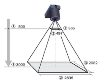
Figure 30: Field of view V2D8512R-xxxxxxxx, focal length: 12 mm
