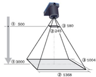
Figure 32: Field of view V2D8512R-xxxxxxx, focal length: 25 mm
