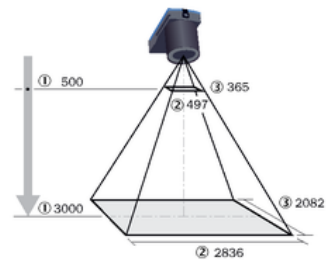
Figure 30: Field of view V2D8512R-xxxxxxxx, focal length: 12 mm
