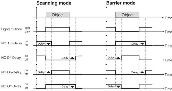
fig. 4 On-Delay and Off-Delay
