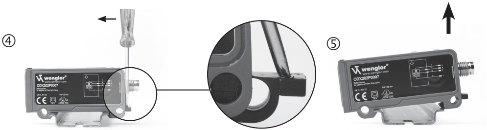
fig.1 Mounting of the Sensor to a DIN rail
