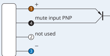
Pinout
