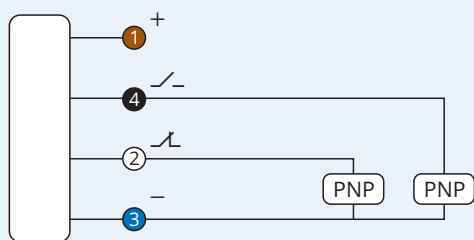
Pinout
