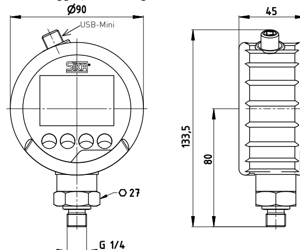
With data logger, measuring cell PIEZO
