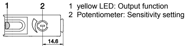
Fig. 1: Display and operating elements
