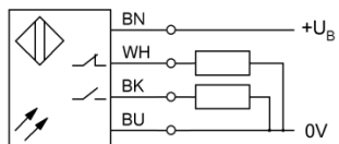
Fig. 14: Connection diagram
