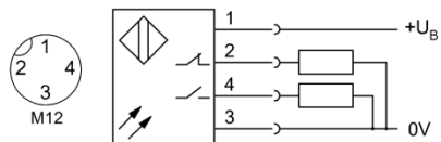
Fig. 13: Pinouts, connection diagram
