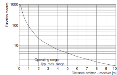
Fig. 15: Function reserve depending on the distance between the emitter and receiver
