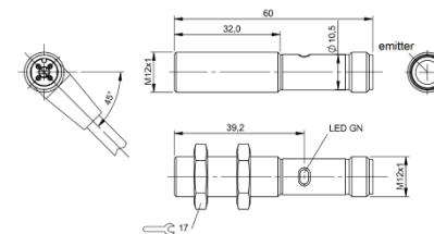
Fig. 7: Dimensions
