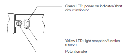
Fig. 5: Display and operating elements (for BOS 12M-PA-RE10-...)
