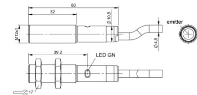
Fig. 8: Dimensions
