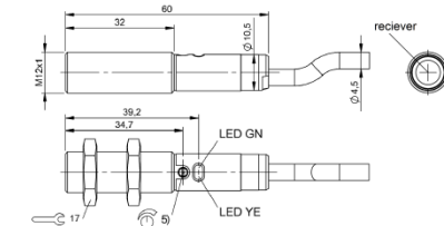
Fig. 10: Dimensions
