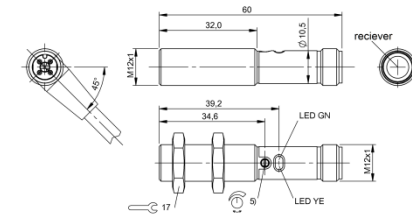
Fig. 9: Dimensions
