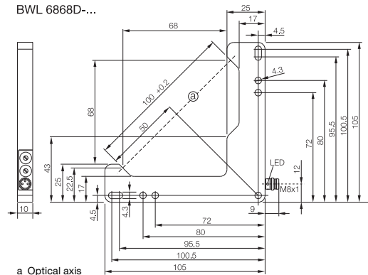
Fig. 5: dimensional drawing
