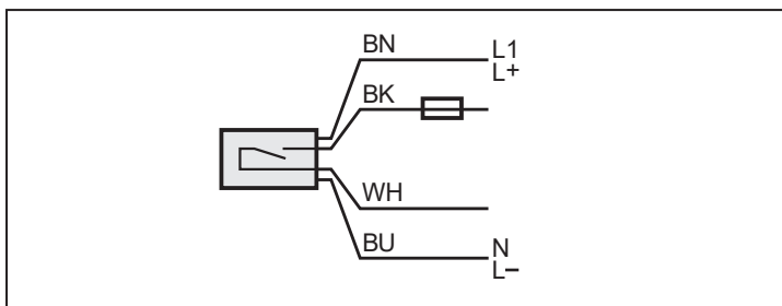
Fig. 4: Wiring diagram (colours to DIN EN 60947-5-2)
